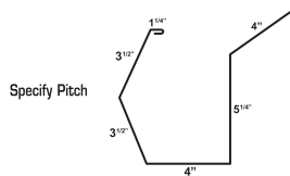
Sculptured Pre Hung Gutter
