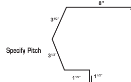
Sculptured High Side Eave
